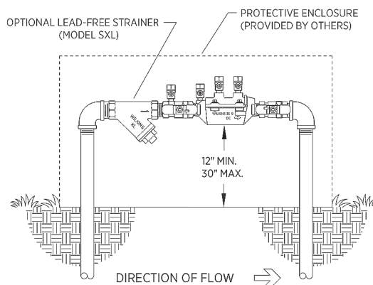
OUTDOOR INSTALLATION
