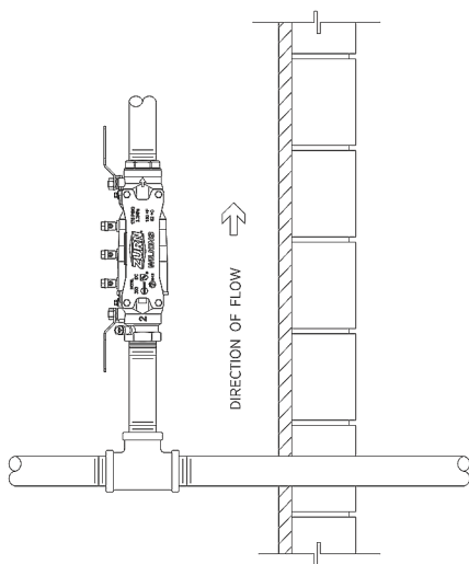
INDOOR INSTALLATION
